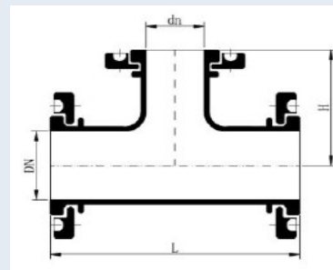
TE BRIDA- BRIDA LOOSING FLANGED TEE
