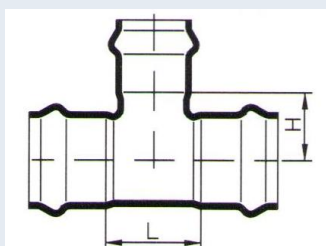
TE ENCHUFE-ENCHUFE-ENCHUFE PVC/ALL SOCKET TEE
